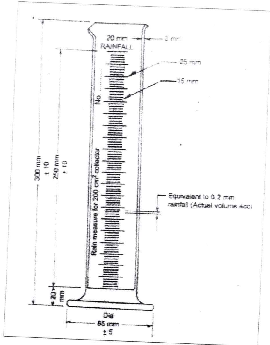
Fig. 15(b) Rain Measure For 200 sq. cm Collector
